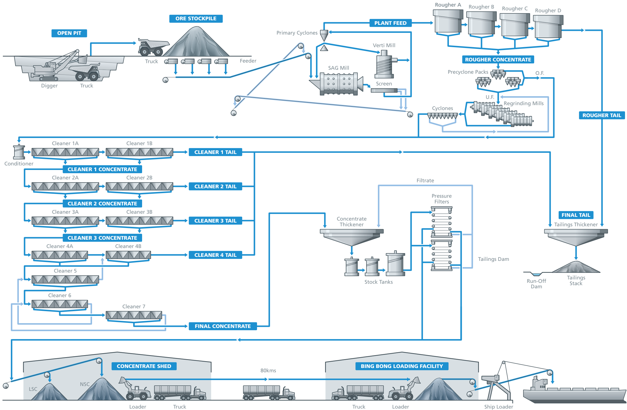
This diagram illustrates the complete mineral processing workflow, from extraction at the open pit to final product handling. The process begins with ore extraction and transport to the stockpile, followed by primary crushing and grinding in SAG and Verti Mills. The resulting slurry is classified through a series of rougher and cleaner stages. The final concentrate is thickened and filtered, while the tailings are thickened and stacked. The concentrate is then transported 80 kilometers to the Bing Bong Loading Facility for shipment via ship loader.
